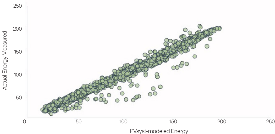
Figure 5 — PVsyst-modeled energy vs. actual energy measured
